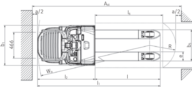
Top view EXH-SF 16C/20C
