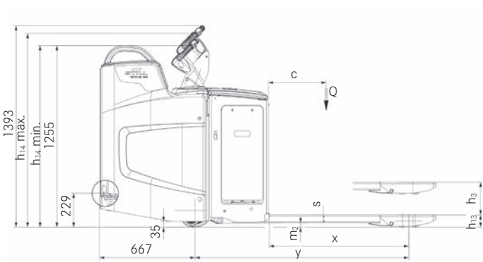
Side view rear entry EXH-S
