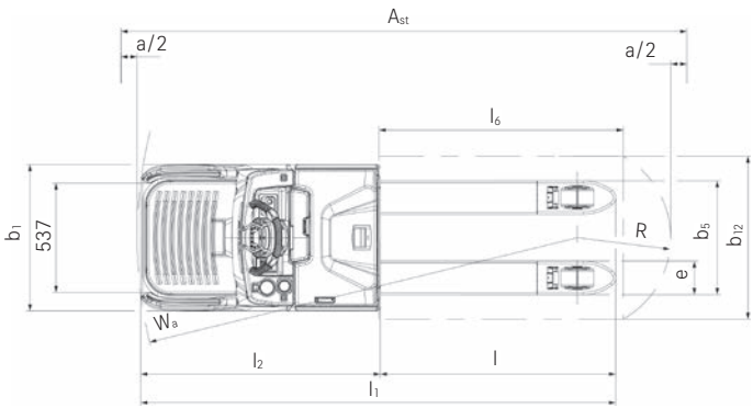
Top view rear entry EXH-S
