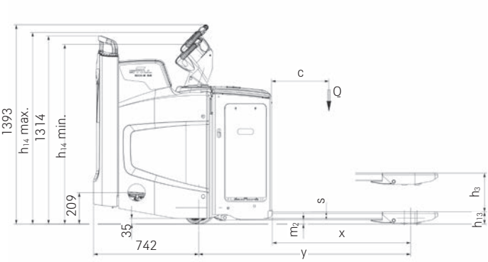
Side view side entry EXH-S
